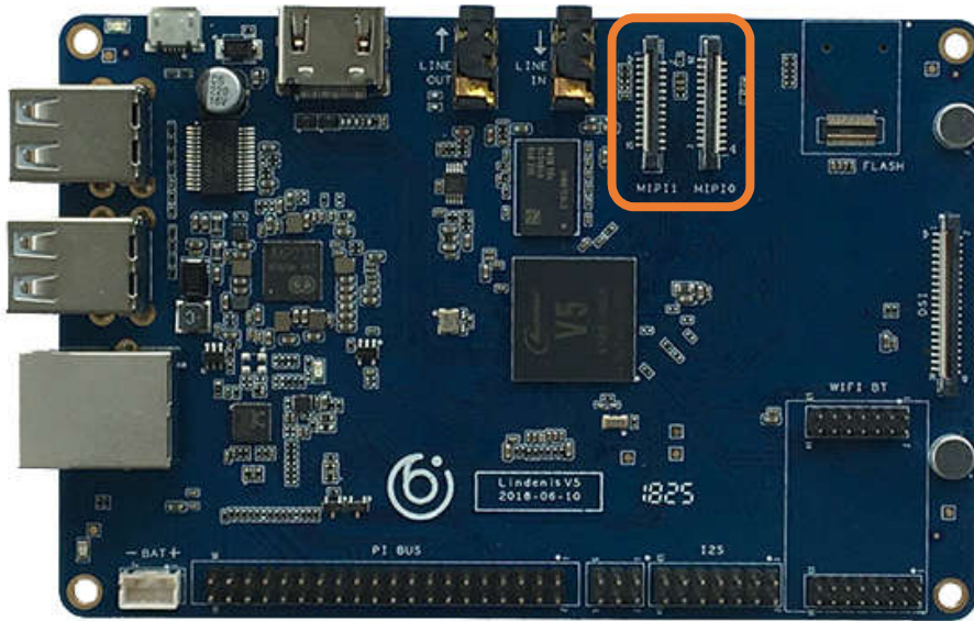
Figure 1: MIPI-CSI Connectors Location (Left: CSI1, Right:CSI0)
