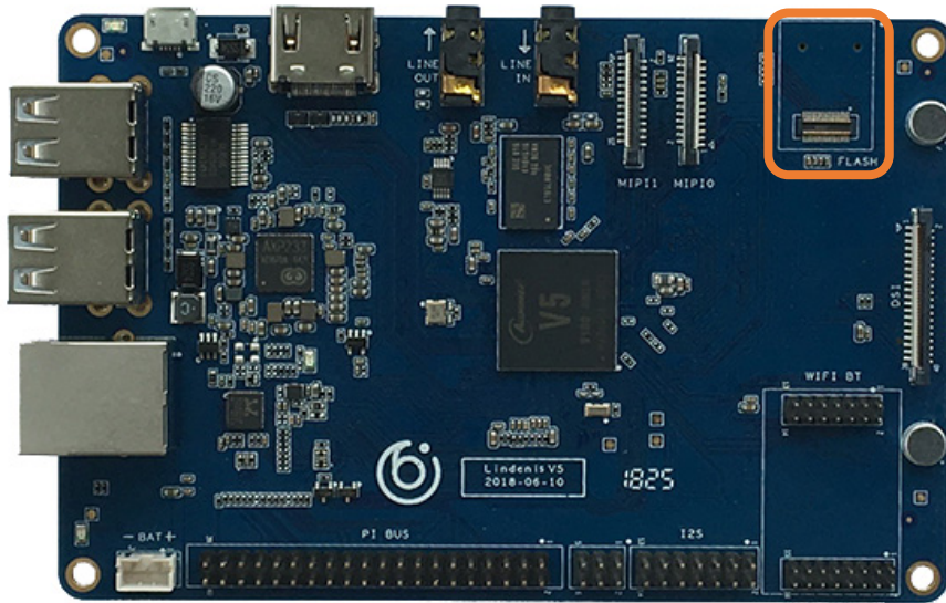
Figure 1: eMMC connector location
